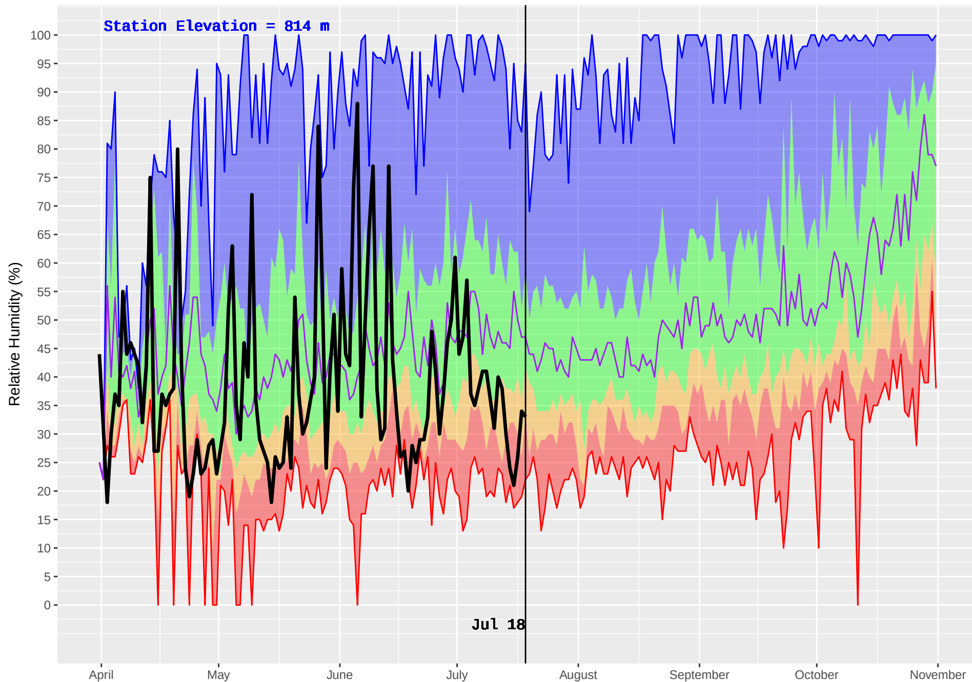
CHILAKO (189) : Historical (1986–2016) and Current (2018) Daily Relative Humidity
