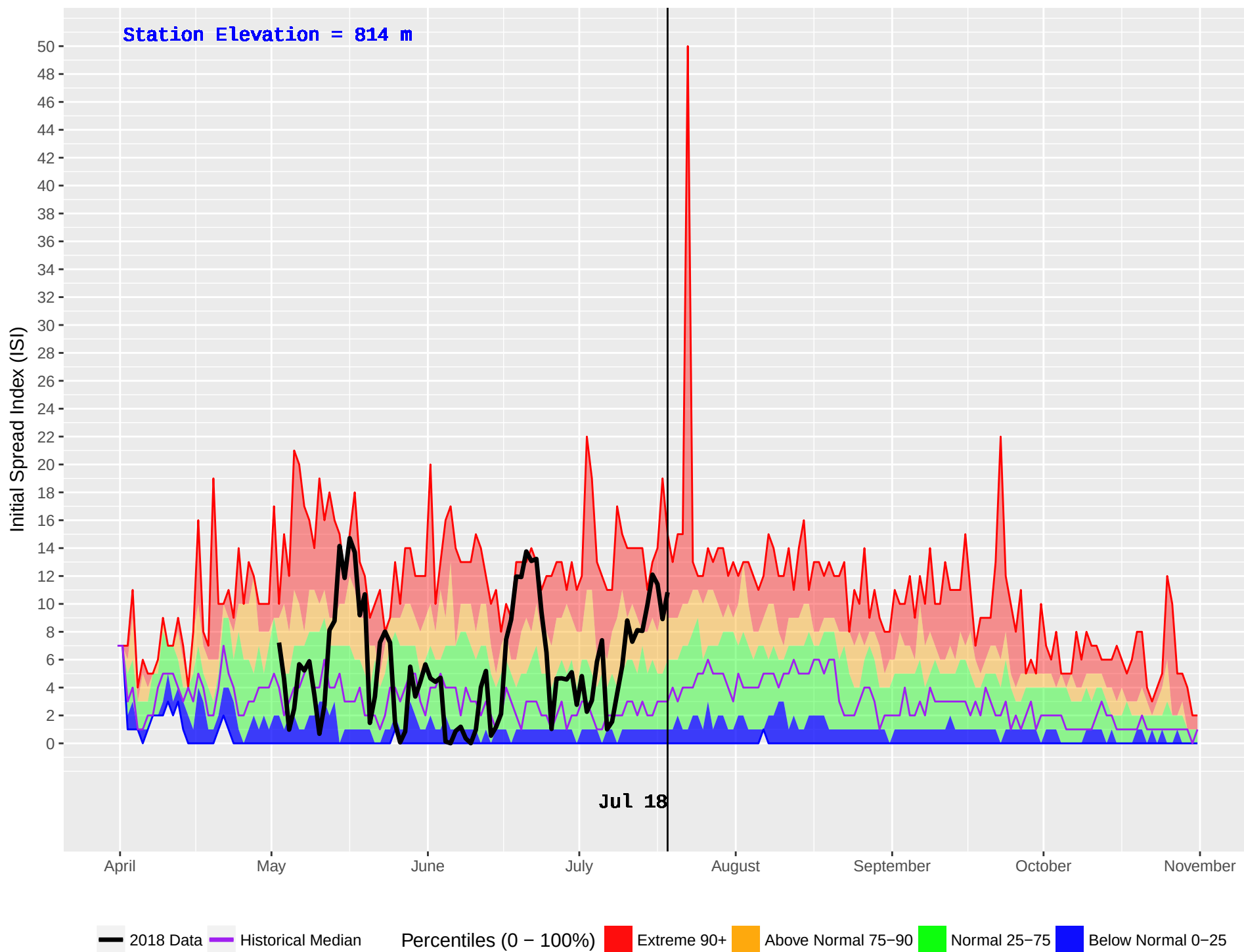
CHILAKO (189) : Historical (1986–2016) and Current (2018) Daily Initial Spread Index (ISI)
