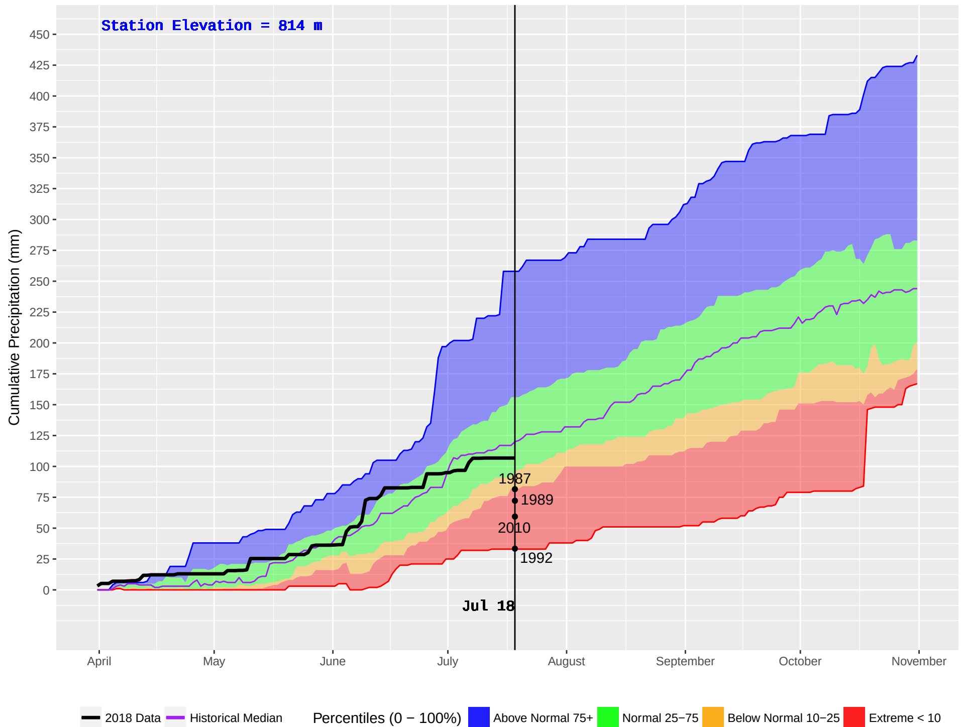
CHILAKO (189) : Historical (1986–2016) and Current (2018) Daily Cumulative Precipitation
