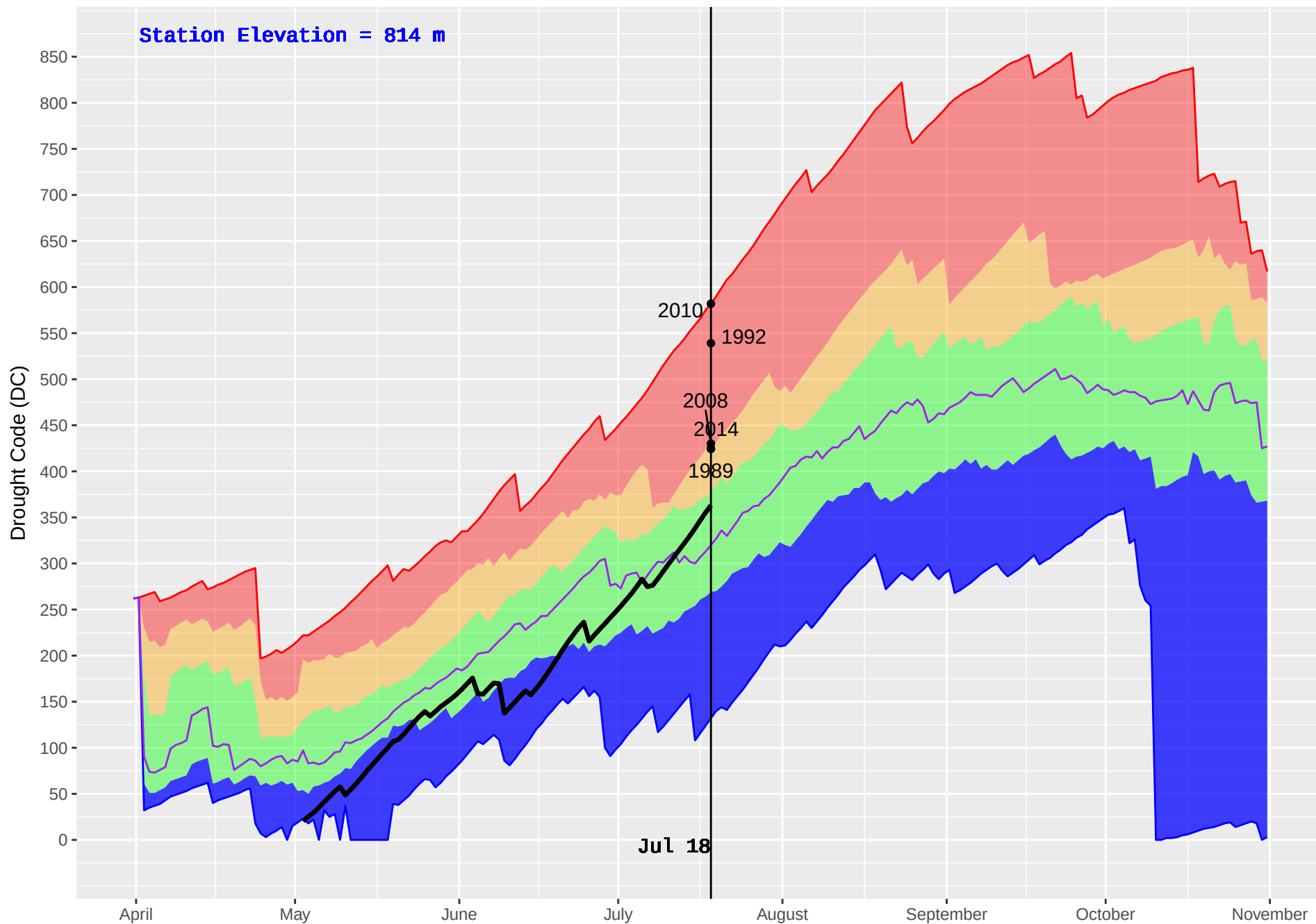
CHILAKO (189) : Historical (1986–2016) and Current (2018) Daily Drought Code (DC)
