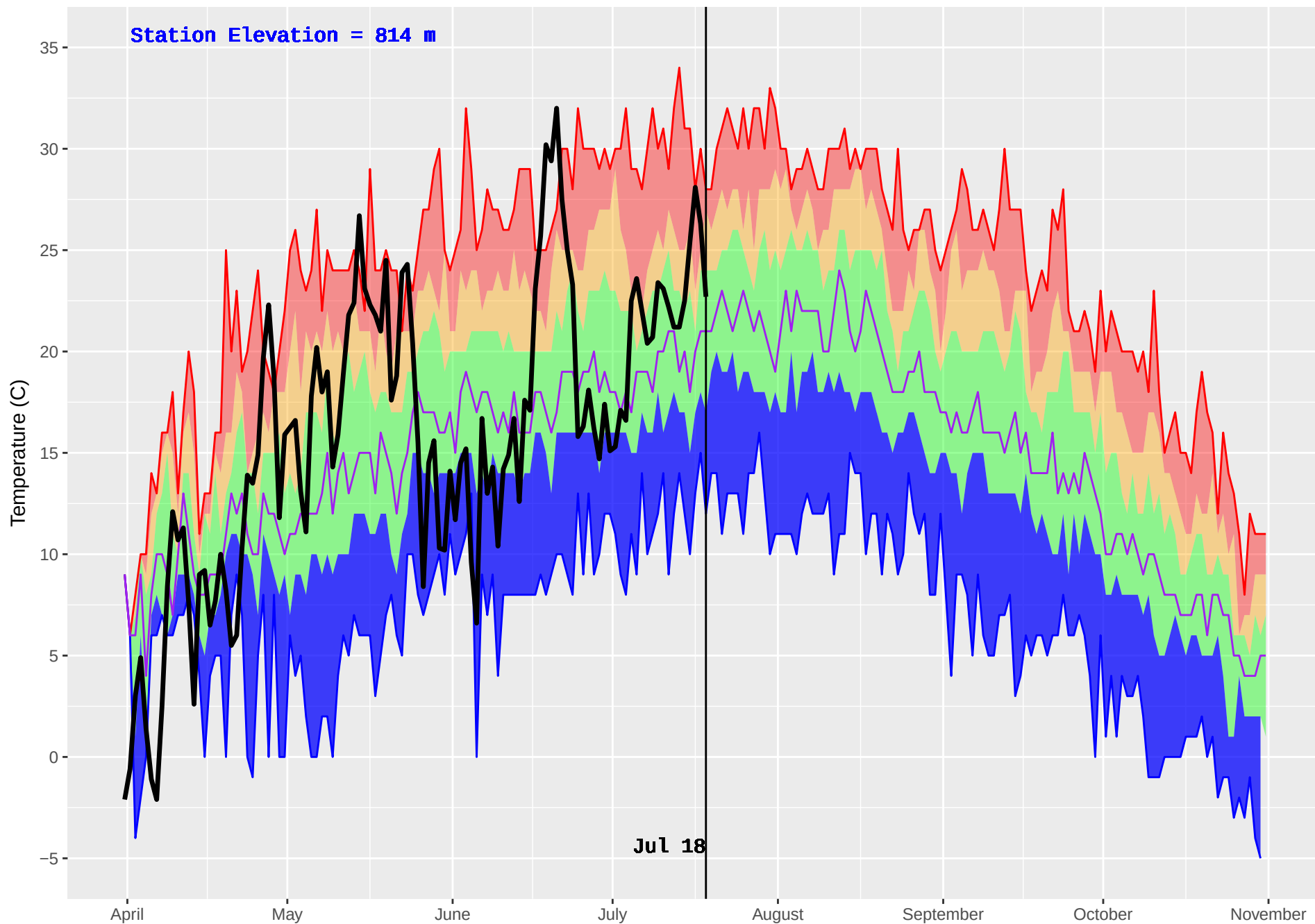
CHILAKO (189) : Historical (1986–2016) and Current (2018) Daily Temperature
