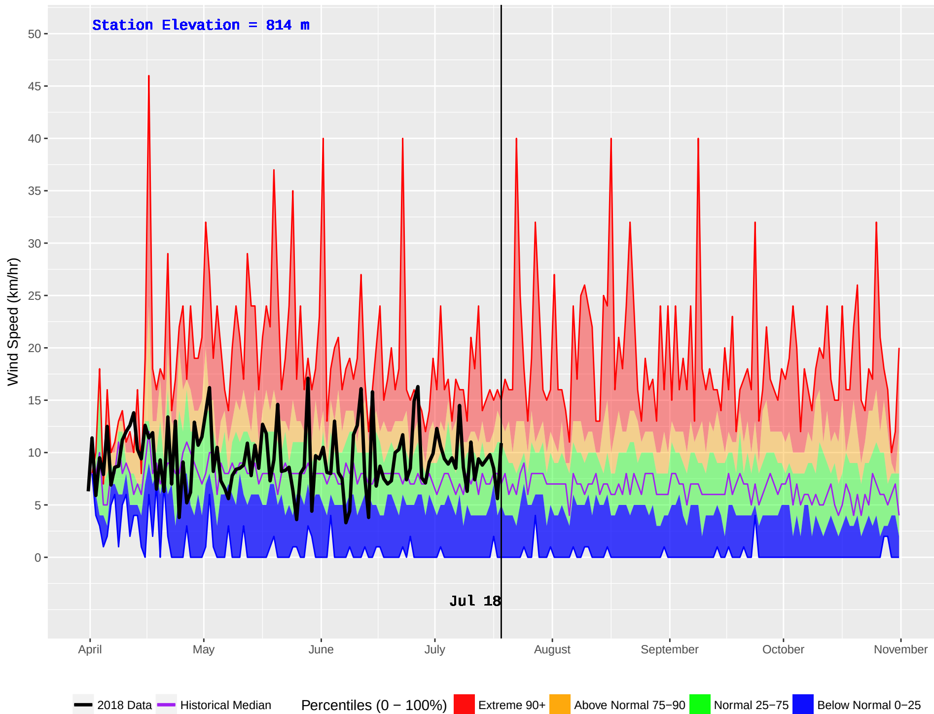
CHILAKO (189) : Historical (1986–2016) and Current (2018) Daily Wind Speed
